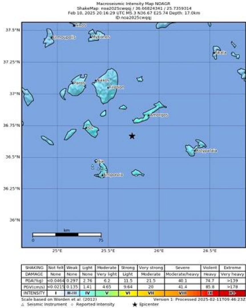
Figure 11: Shakemap of the largest earthquake using the results of the automatically processed accelerograms and the revised hypocenter and magnitude solutions by the analysis team of NOAIG.
