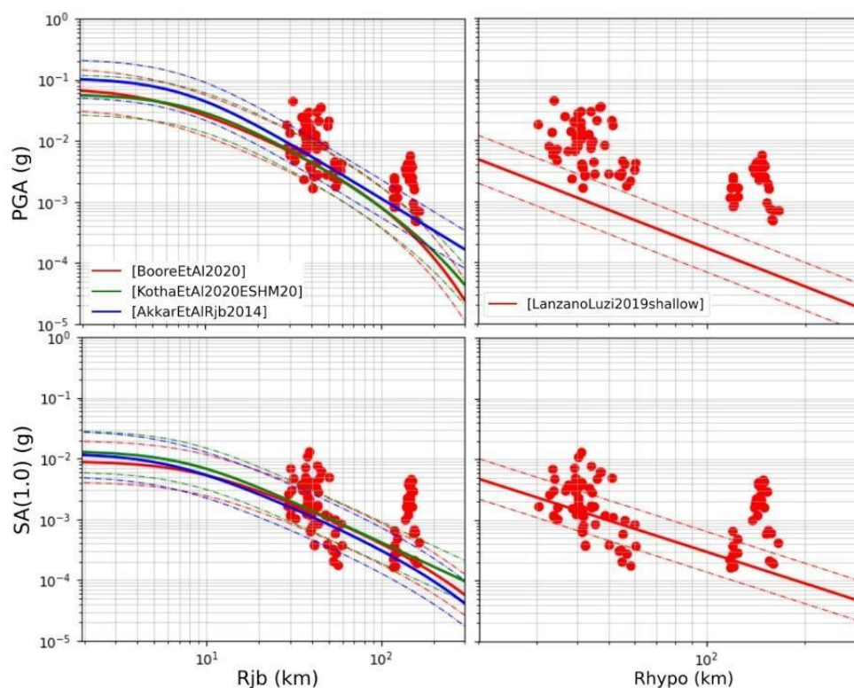
Figure 21: An example of the comparison of observed peak ground acceleration (PGA) values across all the stations studied for earthquakes with magnitudes M4.6-M4.7, with 3 attenuation relationships for shallow tectonic earthquakes (on the left) and 1 relationship for volcanic strong ground motions (on the right).
