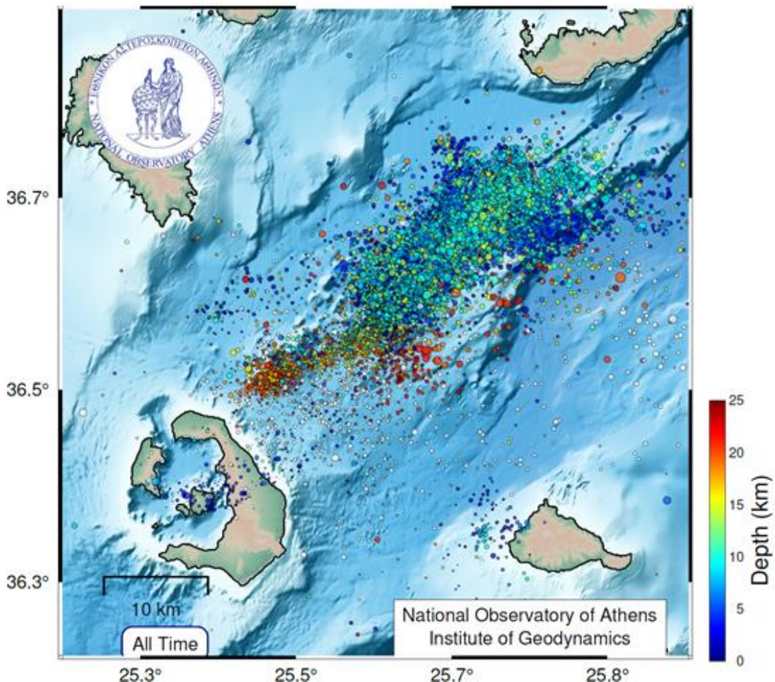
Figure 17: Seismic events that resulted from the application of the EQTransformer algorithm for the period between 1/06/2024 and 05/03/2025 and are characterized by small location errors.
